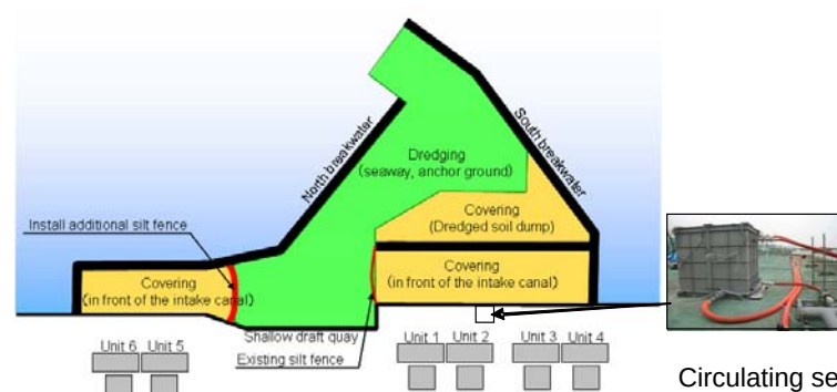
Figure 4: Harbor's Seabed Soil Image
